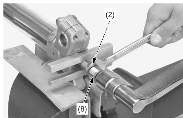
(2) contratuercas (8) perno central
